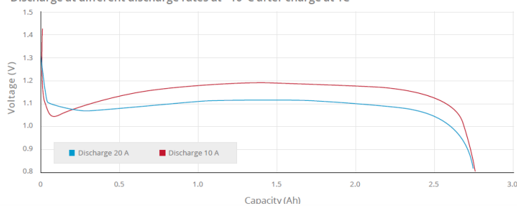
Discharge at different discharge rates at - 10°C after charge at 1C
