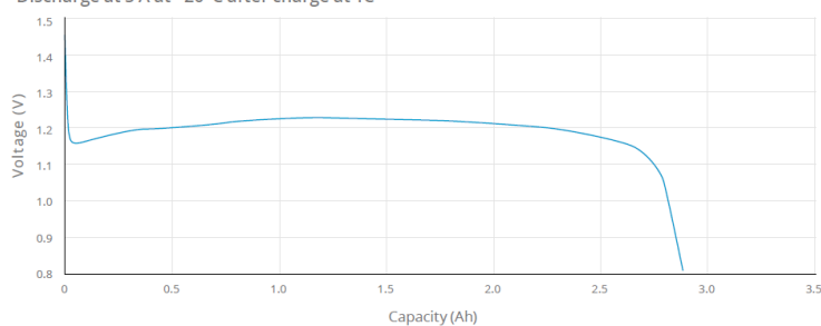
Discharge at 5 A at - 20°C after charge at 1C
