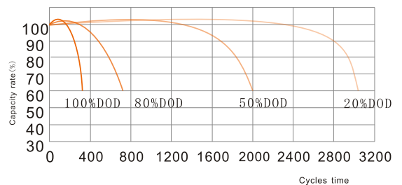
Cycle life curves (25°C) / Courbes de cycle de vie (25°C) Discharge at 0.1C / Cut off voltage 1.8V by cell
