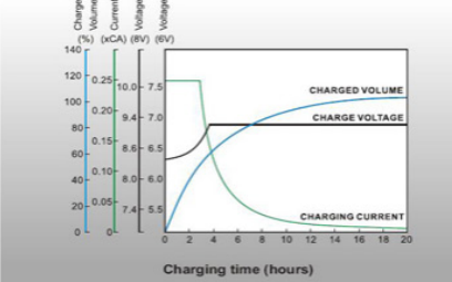
Constant voltage charging characteristic (0.25CA, 25°C, 77°F)
