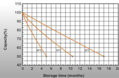
Self-discharge characteristic
