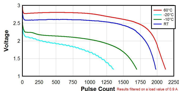
0.9 Amp, 3 sec ON / 27 sec OFF @ Various Temperatures
